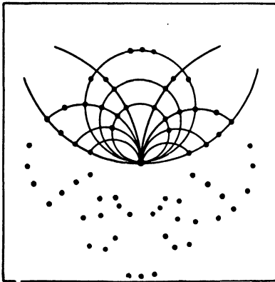
FIG. 5.—Elliptical loci of spots of Laue pattern.
